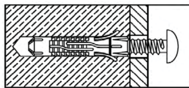
Install anchor.
