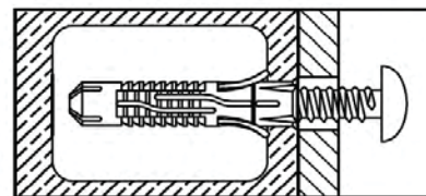
Install anchor.
