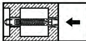
Install anchor.
